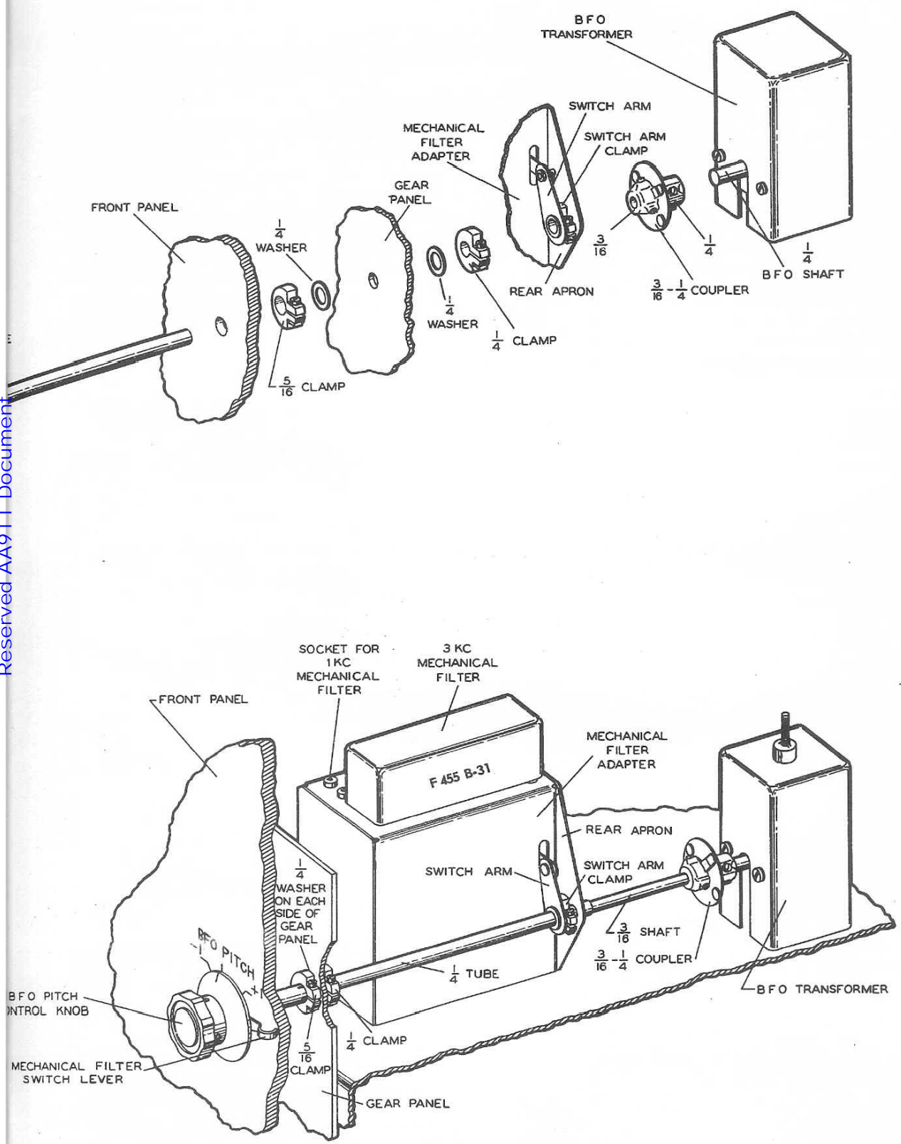
Figure 2. Mechanical Assembly
