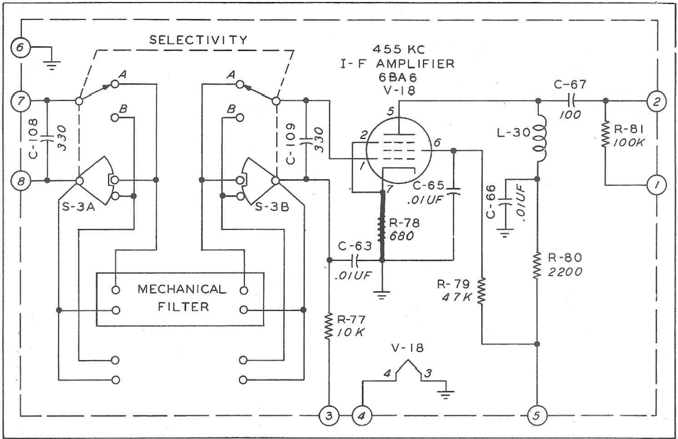
Figure 5. Mechanical Filter Adapter Schematic
