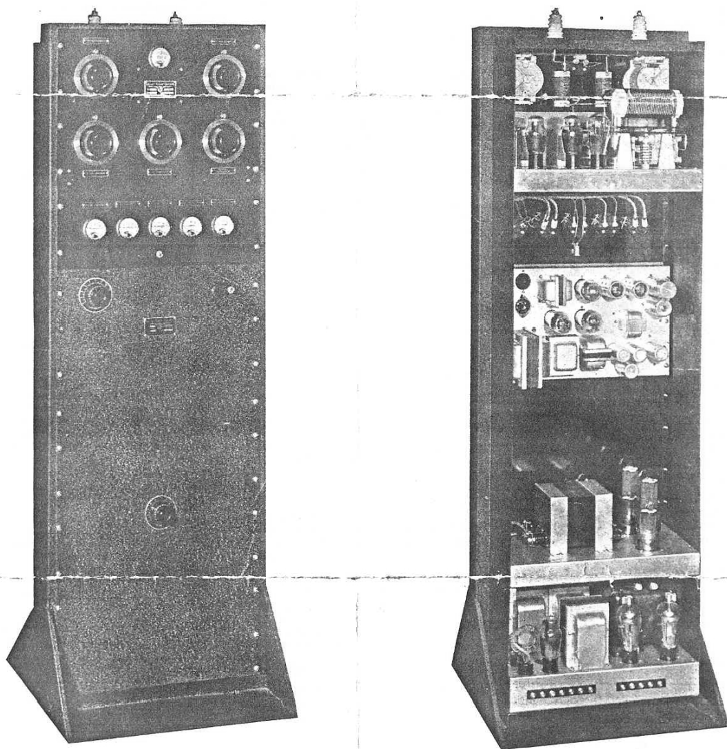
FRONT AND REAR VIEWS OF COLLINS 30 FXB TRANSMITTER
