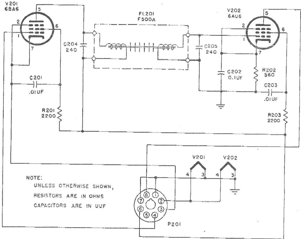
Figure 1. 353C Series Adapter Schematic
