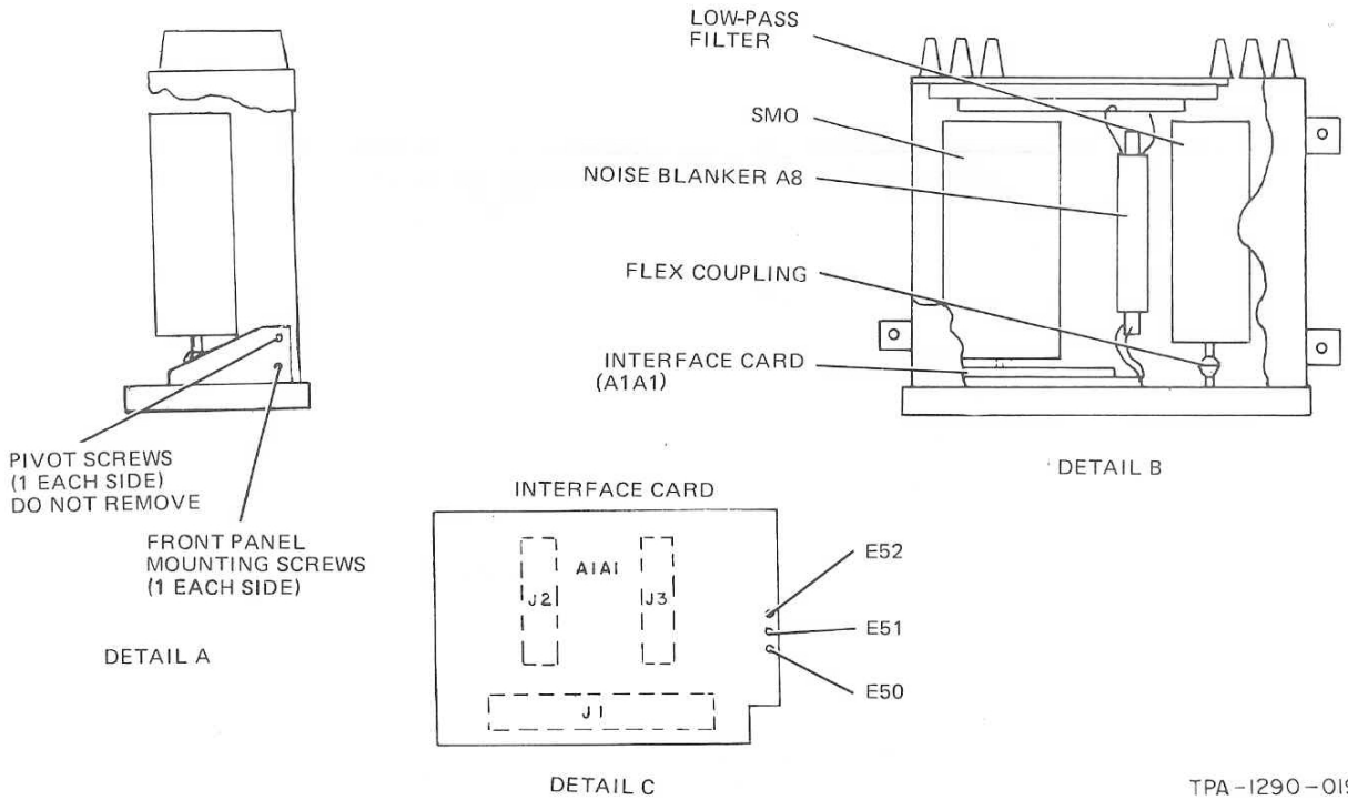
HF-281/HF-282 Component Locations Figure 3
